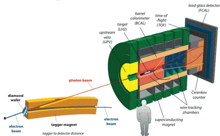
Fig. 1: Illustration of the relative position of the source of polarized photons (diamond wafer), GlueX target, and surrounding components making up the high energy physics detector. [image from www.gluex.org]
