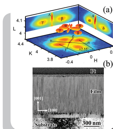
Fig. 1: (a) The H-K, H-L, and K-L cross-sectional RSM measured around the asymmetric (0 4 4) reflection, with L = 4.08 . The \alpha and \delta peaks are orthorhombic phases, while the \beta and \gamma peaks are rotated tetragonal phases associated with the CB structure. The elastically strained tetragonal phase is labeled A. Signal originating from domain boundaries, highlighted by the radial lines emanating from the central (0 4 4) RLP, are labeled \rho , \sigma , \tau and \nu . The central figure is a 3D reconstruction of experimentally determined FWHMs of the corresponding peaks. Reprinted figure with permission from Reference [6]. Copyright (2008) by the American Physical Society. (b) TEM image of the CB film on MgO substrate.
